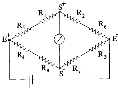
Fig. 3. Strain-gauges Wheatstone bridge network
