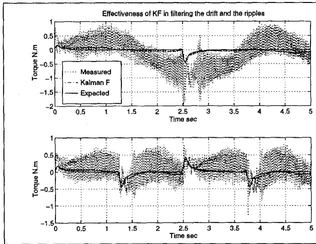
Fig. 10. Kalman filter performance to cancel torque ripples, and misalignment torque for two typical experiments
