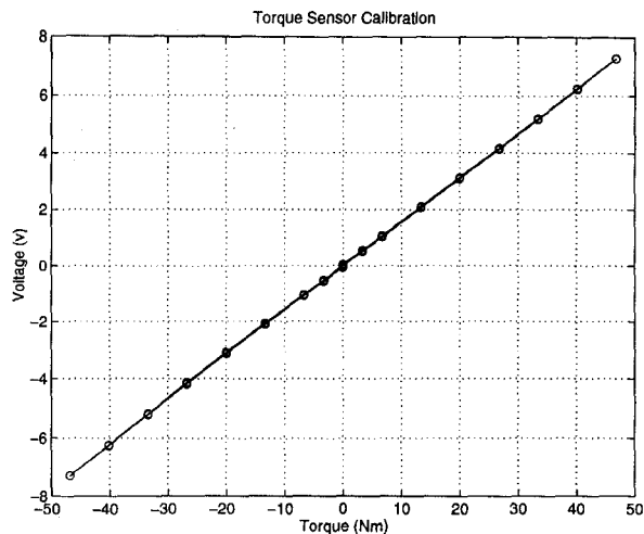
Fig. 6. Torque sensor calibration results for full-range loading
