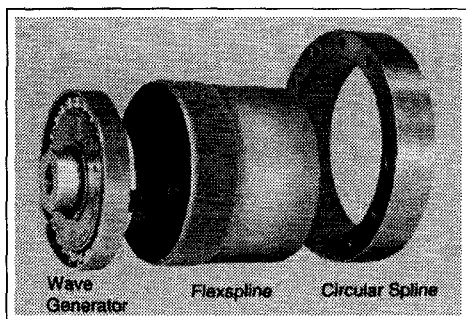
Fig. 1. Harmonic drive components
