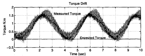
Fig. 9. Misalignment torque signature on the measured torque
