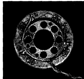
Fig. 5. Harmonic drive built-in torque sensor
