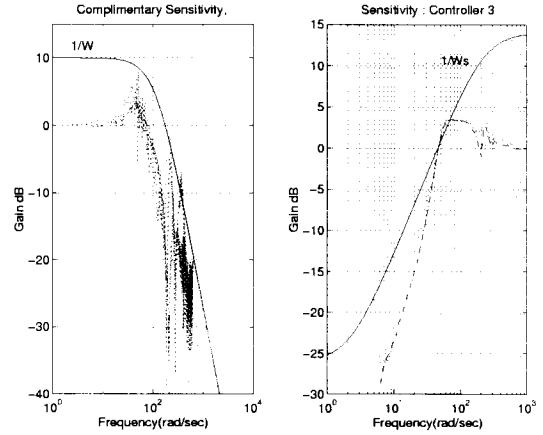
Fig. 2. Closed-loop frequency performance
