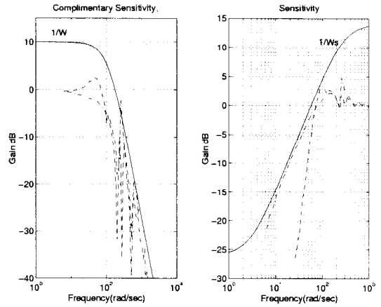
Fig. 7. Closed-loop frequency performance comparison of the system with and without friction-compensation; Dashed : With friction-compensation, Dash-Dotted : Without friction-compensation
