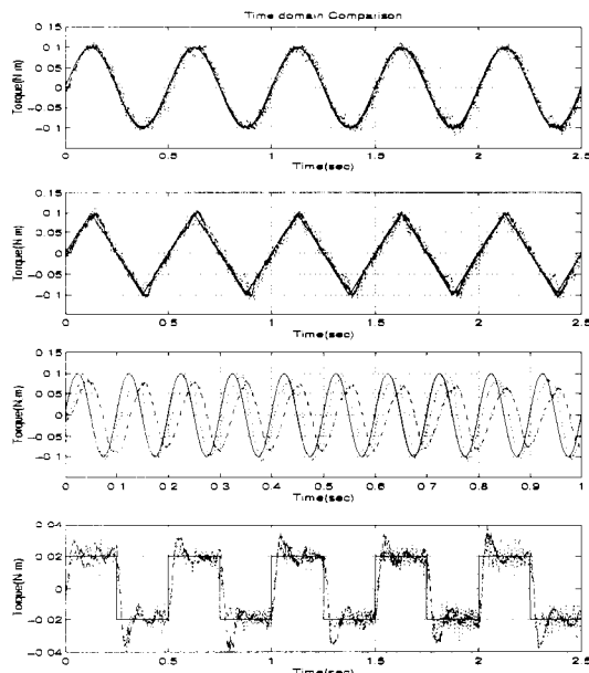
Fig. 8. Closed-loop time response comparison of the system with and without friction-compensation; Solid : Reference command, Dash-Dotted : With friction-compensation, Dotted : Without friction-compensation
