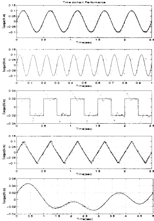
Fig. 3. Closed-loop time performance of the system employing Kalman filtered torque and robust controller
