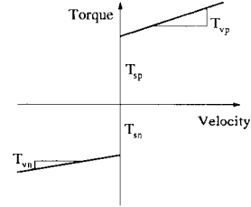
Fig. 4. Identified Coulomb and viscous friction curve for harmonic drive systems
