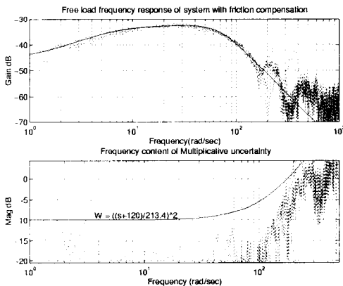
Fig. 6. Frequency response of the free-motion system with friction compensation, its nominal model, and multiplicative uncertainty
