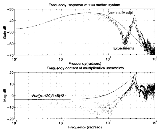
Fig. 1. Frequency response of the system, nominal model, and multiplicative uncertainty
