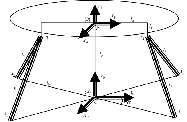
Figure 2: A geometric model for the hydraulic shoulder manipulator
